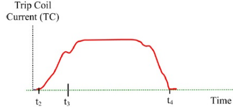
Fig. 2. Trip coil current during opening
