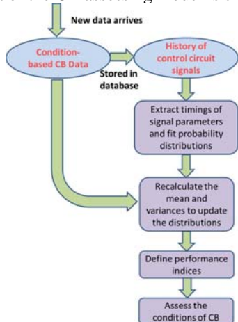
Fig. 4. Model flowchart for assessing the CB conditions
