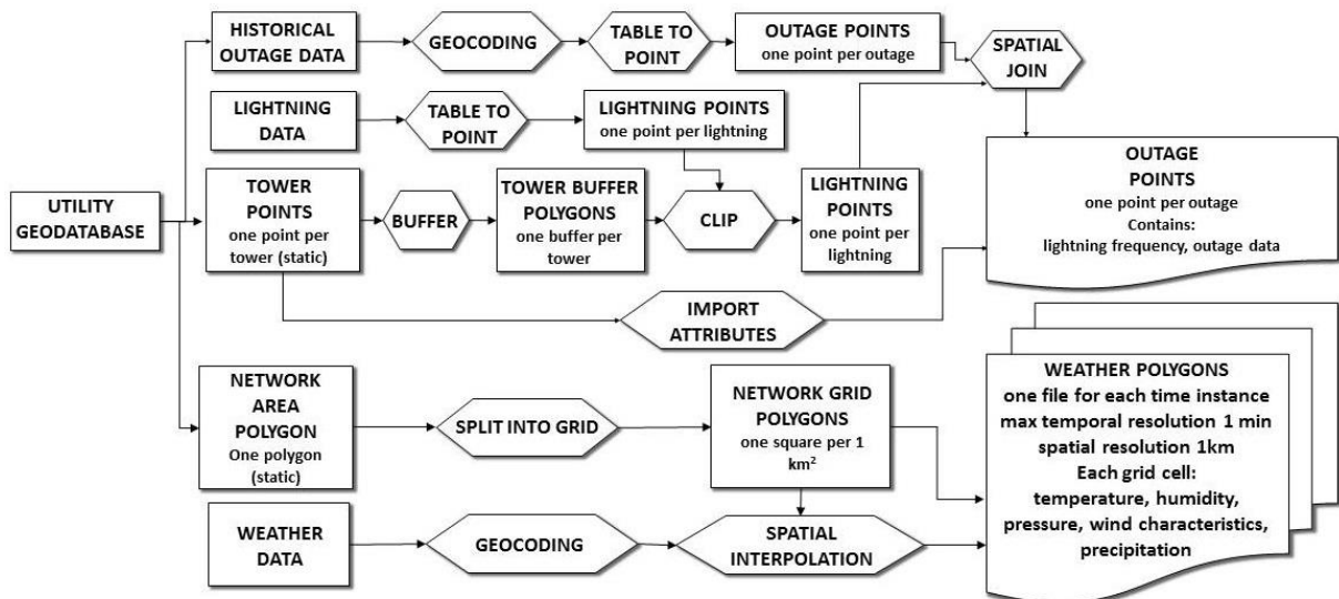
Figure 4. Spatial Correlation of Data
