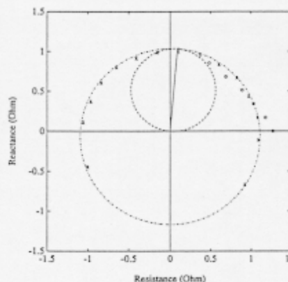
'-----': Theoretical steady-state characteristic '- - - -': Theoretical dynamic characteristic 'x': Test results using one-terminal model 'o': Test results using two-terminal model
