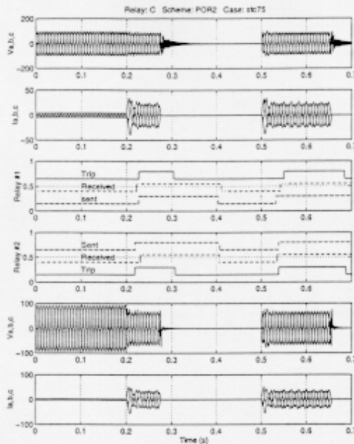
Fig.12 A typical graphical two-terminal test result for Relay C
