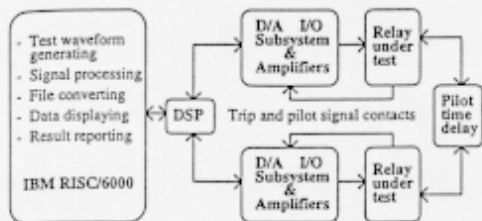
Fig.4 Two-terminal testing set up
