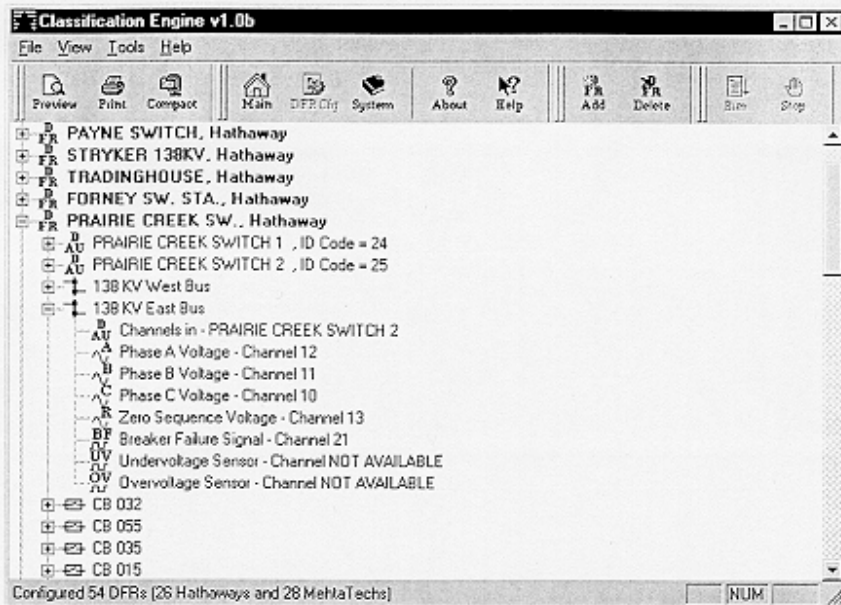
Figure 6. The Classification Engine configuration display
