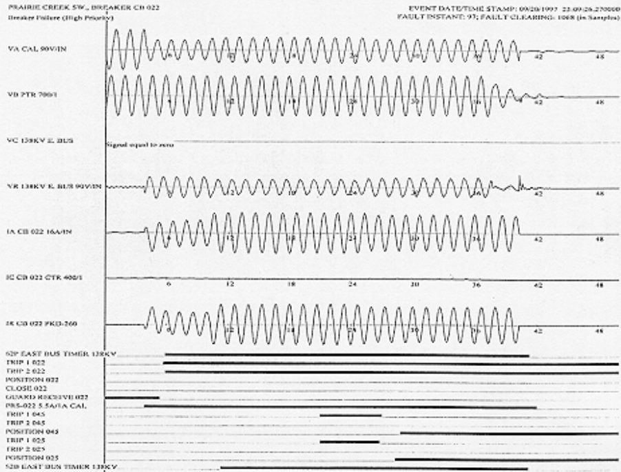
Figure 13. The paper printout generated by the Report Viewer software
