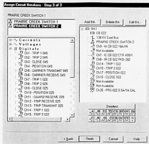
Figure 5. DFR configuration wizard
