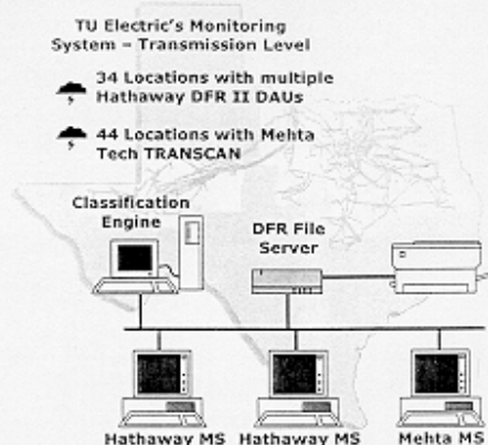
Figure 2. TU Electric's Classification System
