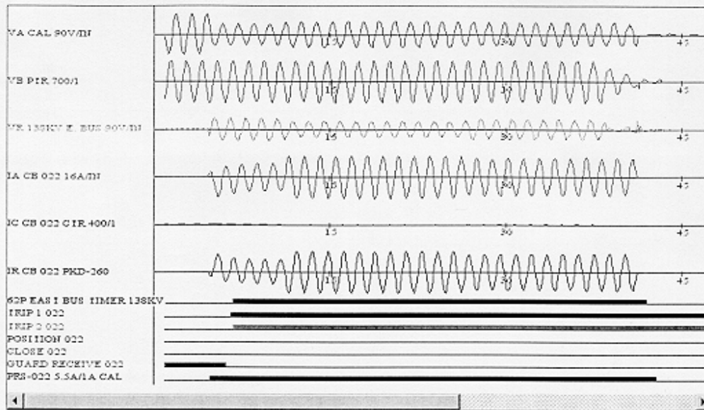
Figure 12. The Report Viewer waveform display
