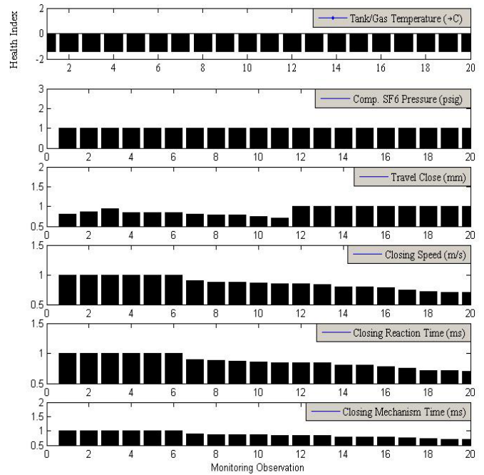
Fig. 7. Health status of monitored parameters for CB#4 closing operation.
