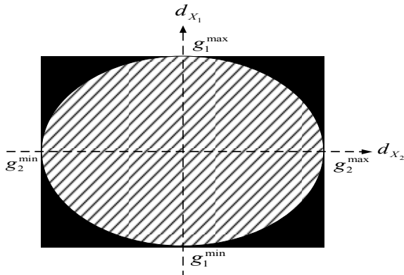
Fig. 3. Two-dimensional example of an inscribed hyper-ellipse
